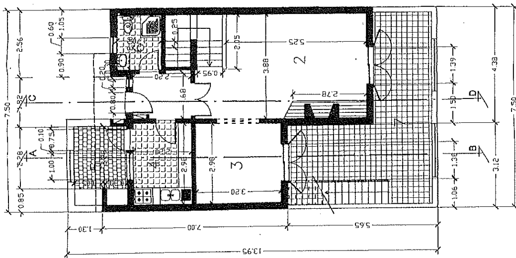
PLANTA DO RES-DO-CHÃO Ground Floor
