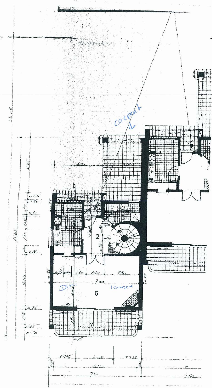
PLANTA DO R/CHÃO / Ground floor
