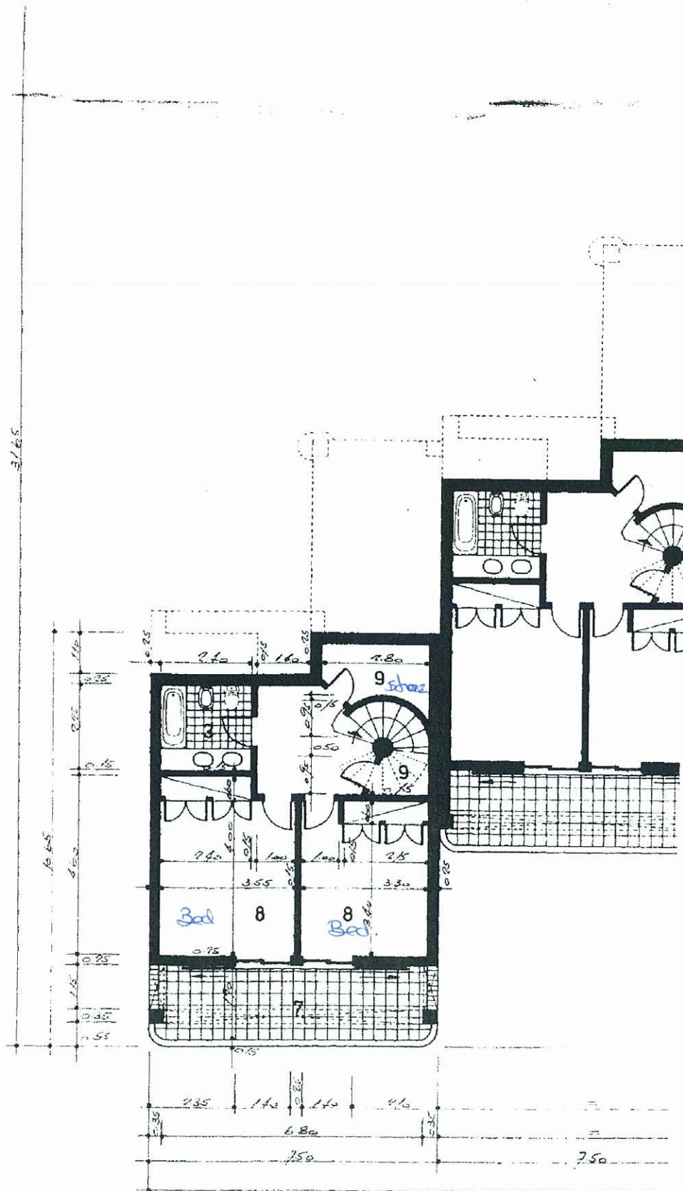
PLANTA DA CAVE / Basement /
